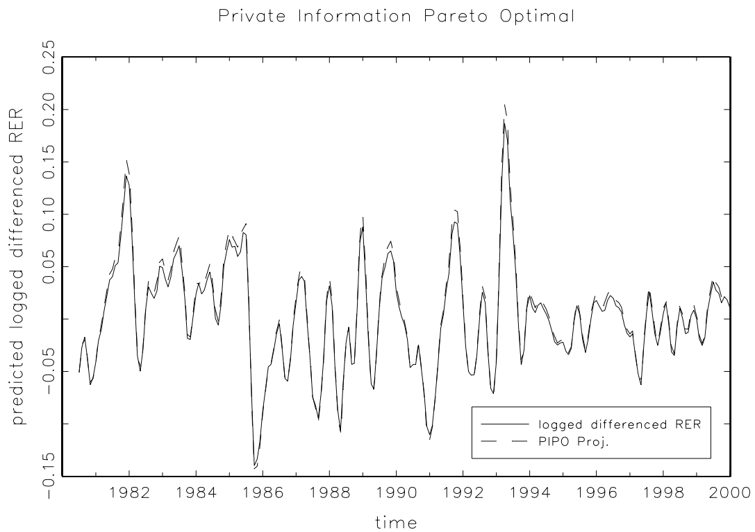
Figure 1: To construct this graph, we regressed the first difference of the log of the PIPO SDF ratio on the first difference of the log of the real exchange rate. We then plot the resultant projection and first difference of the log of the real exchange rate against time.
