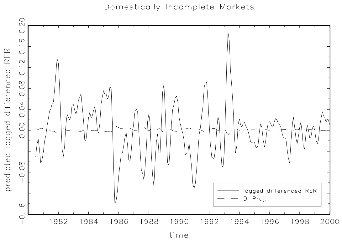
Figure 2: To construct this graph, we regressed the first difference of the log of the DI SDF ratio on the first difference of the log of the real exchange rate. We then plot the resultant projection and first difference of the log of the real exchange rate against time
