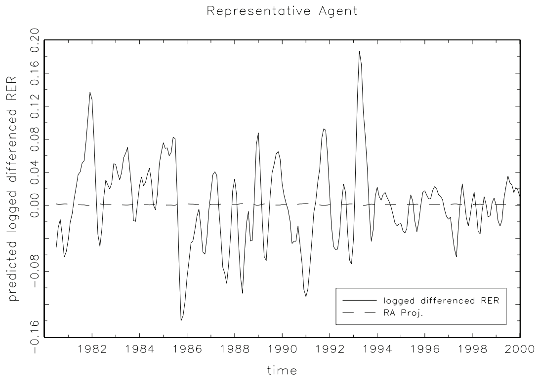
Figure 3: To construct this graph, we regressed the first difference of the log of the RA SDF ratio on the first difference of the log of the real exchange rate. We then plot the resultant projection and first difference of the log of the real exchange rate against time
